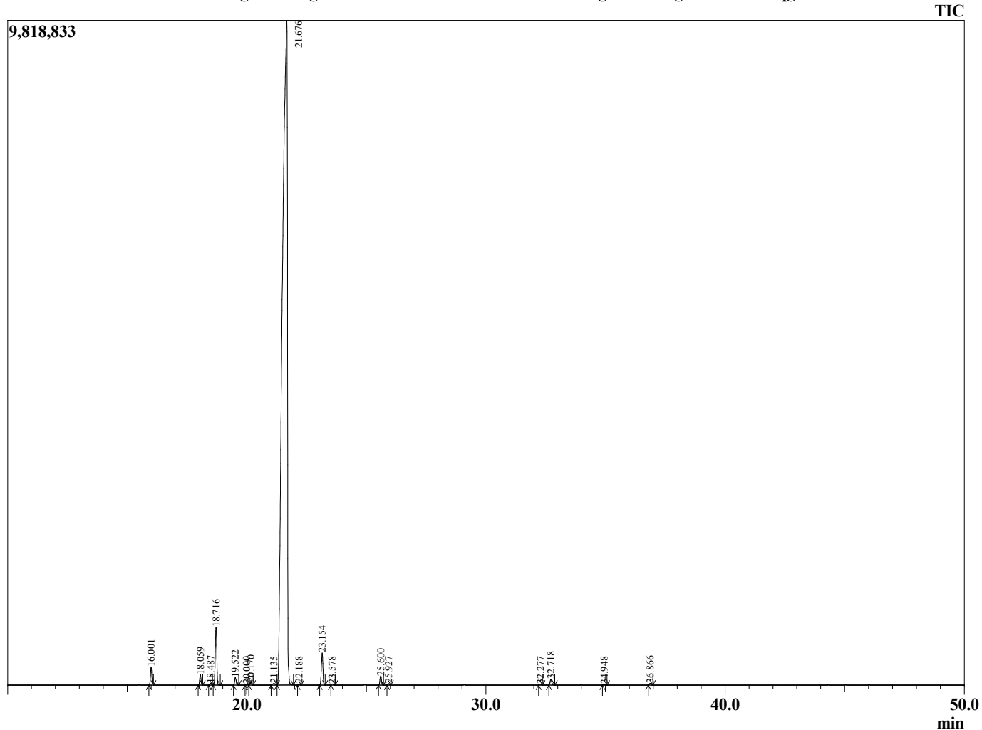
Chromatogram Tangerine C:\GCMSsolution\Data\EOU\Tangerine\Tangerine 141022.qgd
